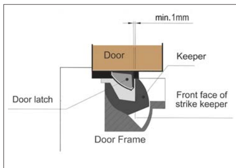
Mechanical door lock configuration
